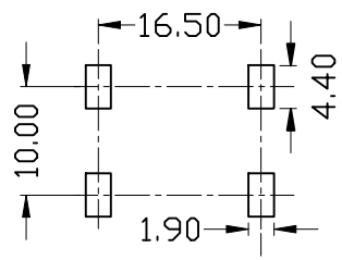
(MOUNTING DETAIL)
