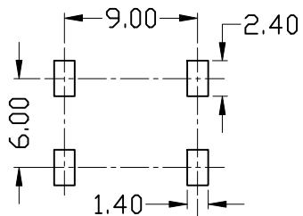
(MOUNTING DETAIL)
