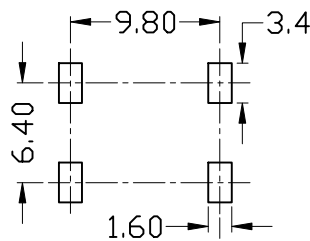
(MOUNTING DETAIL)
