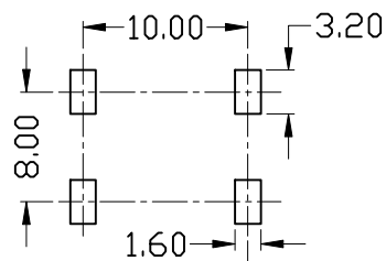
(MOUNTING DETAIL)
